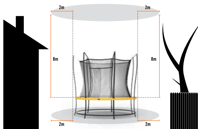
Correct Installation
